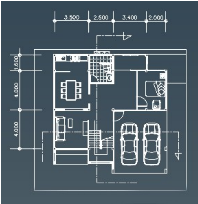
1ST FLOORPLAN
