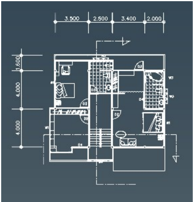
2ND FLOORPLAN
